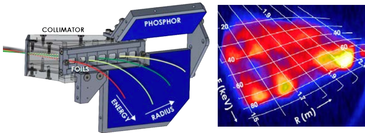
A novel Imaging Neutral Particle Analyzer measures neutralized fast ions escaping from the DIII-D tokamak plasma
