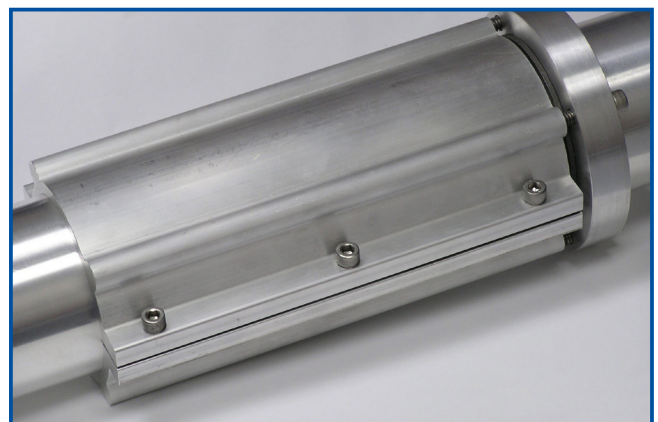
Light weight extruded coupling for 2.5" waveguide
