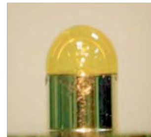
Assembled cryo target with double hemi shell.
