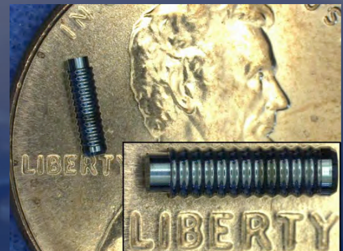
Be rippled rod for SNL Z-machine experiments
