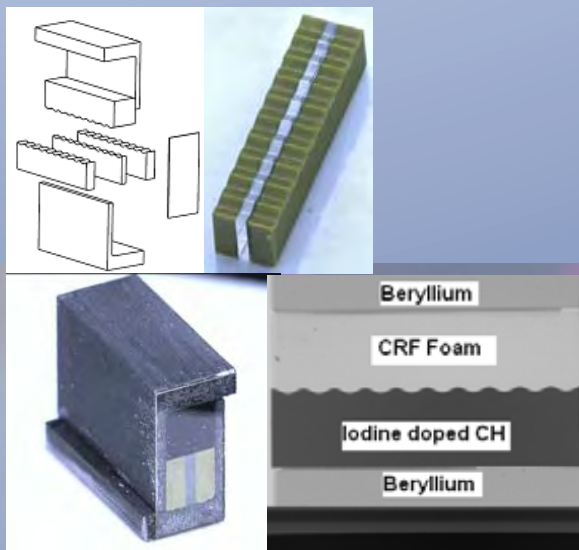
(a) Exploded view of target design (b) Polyamide-imide/CHI sandwich (c) Isometric view of assembled KH target (d) X-radiograph of low-density to high-density mated surfaces.
