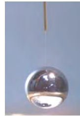
NIF beryllium capsule fill tube assembly showing a 2 mm shell with a 10 \mu m fill tube.
