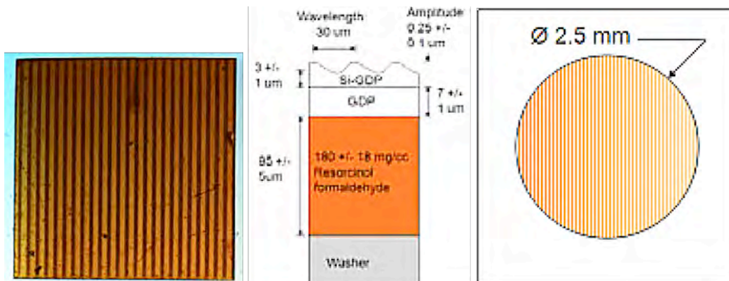
Si-doped and un-doped multi-layer system: GDP/CH/RF/washer \lambda = 30, 60, 120 \mu\text{m} .
