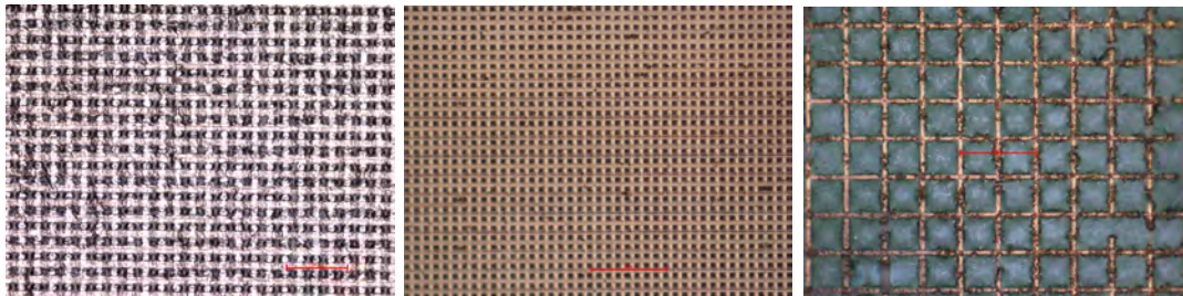
GA 3D printed metal grids in silver (L, C) and gold (R). The individual strands are approximately 2 \mu\text{m} thick
