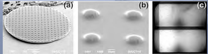
(a) CH flat foil target with square array of bumps. (b) Bumps are nominally 12 \mu\text{m} tall, 25 \mu\text{m} FWHM, and spaced 125 \mu\text{m} apart on a 60 \mu\text{m} thick CH disk. (c) Experimental radiograph from OMEGA shot.
