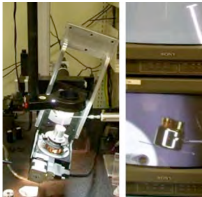
Assembly station in use at SNL.
