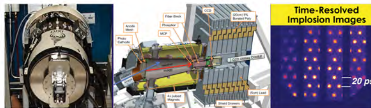
Dilation X-ray Imager (DIXI) system with 20 picosecond temporal resolution
